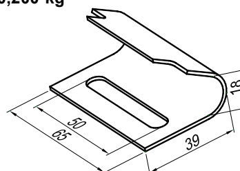
Gancio inox Spessore 3 mm Stainless steel hooks thickness 3 mm
