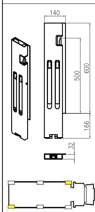
Piantone posteriore PPS Dx PPS rear pillar Right Art. 35406101 - 11,8 kg
