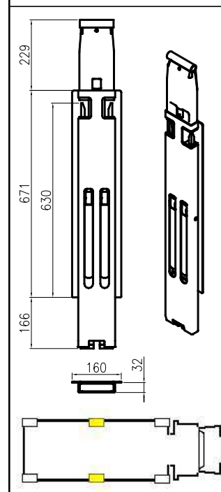
Piantone Kinetop Kinnetop pillar Art. 35408231 - 15,0 kg
