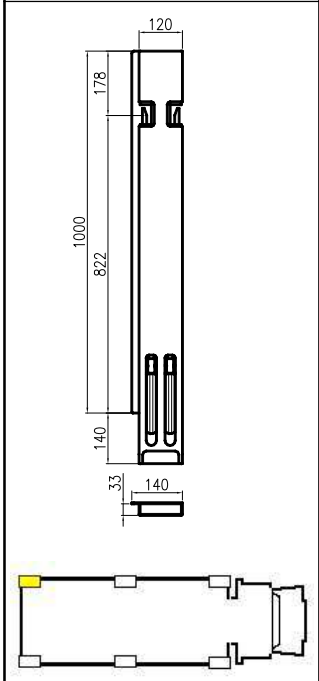
Piantone posteriore Sx Rear pillar Left Art. 35163102
