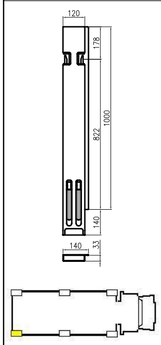
Piantone posteriore Dx Rear pillar Right Art. 35163101
