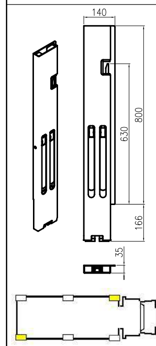
Piantone posteriore PPS Dx PPS rear pillar Right Art. 35408101 - 13,4 kg
