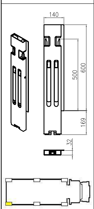
Piantone posteriori PPD Dx PPD rear pillar Right Art. 35406801 - 11,6 kg
