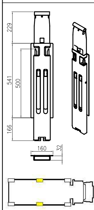
Piantone Kinnetop Kinnetop pillar Art. 35406231 - 13,4 kg
