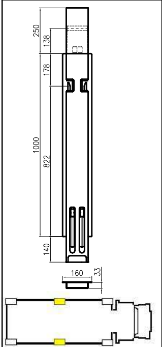
Piantone Centrale Top Hight Top Central pillar Art. 35063120
