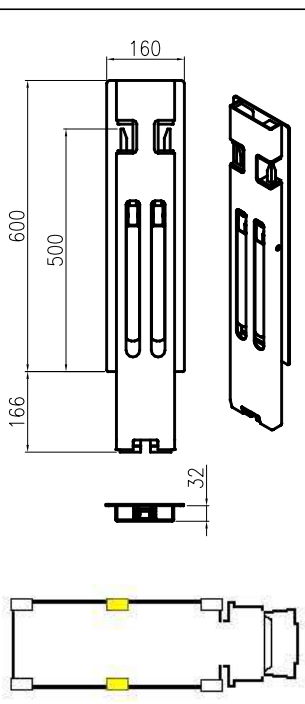
Piantone Centrale Central pillar Art. 35406201 - 12,0 kg
