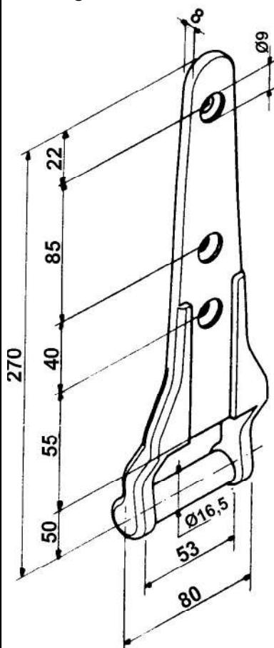
Supporto grezzo Heavy raw Support
