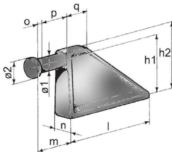
Piantone Pillar
